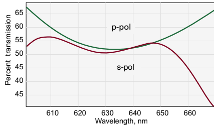
Typical transmission curve @ 633 nm
