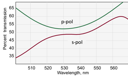
Typical transmission curve @ 532 nm
