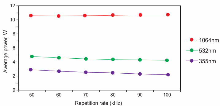
Typical output power for set of repetition rates
